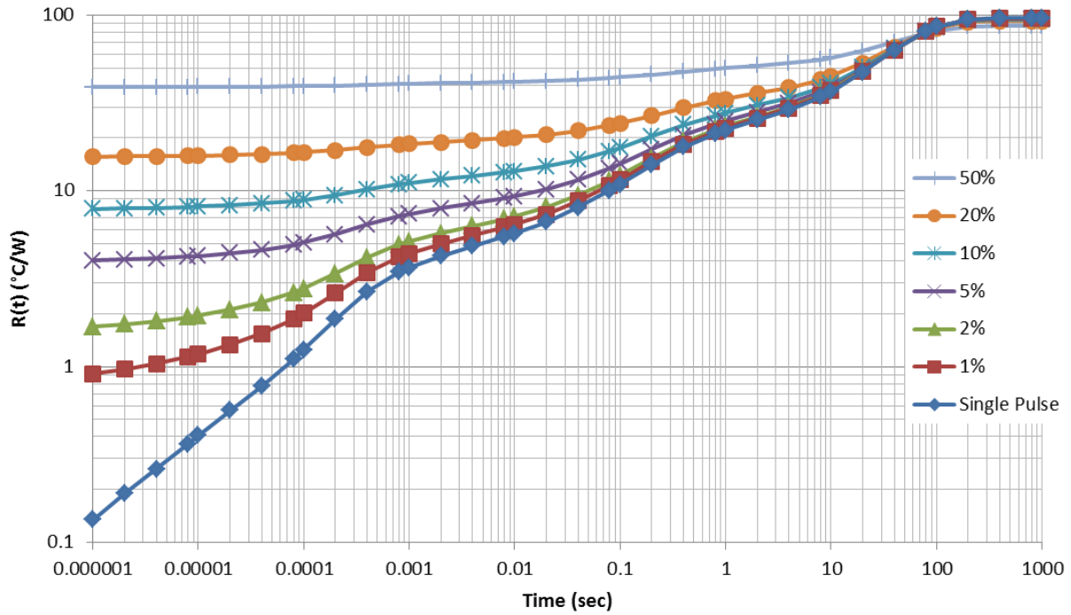
Figure 16. SOIC-14 Thermal Duty Cycle Curve on 645 mm2 Spreader Test Board (1s0p)
