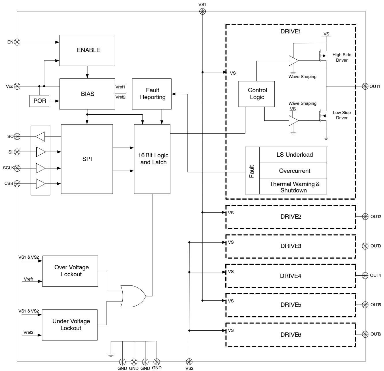
Figure 2. Block Diagram
