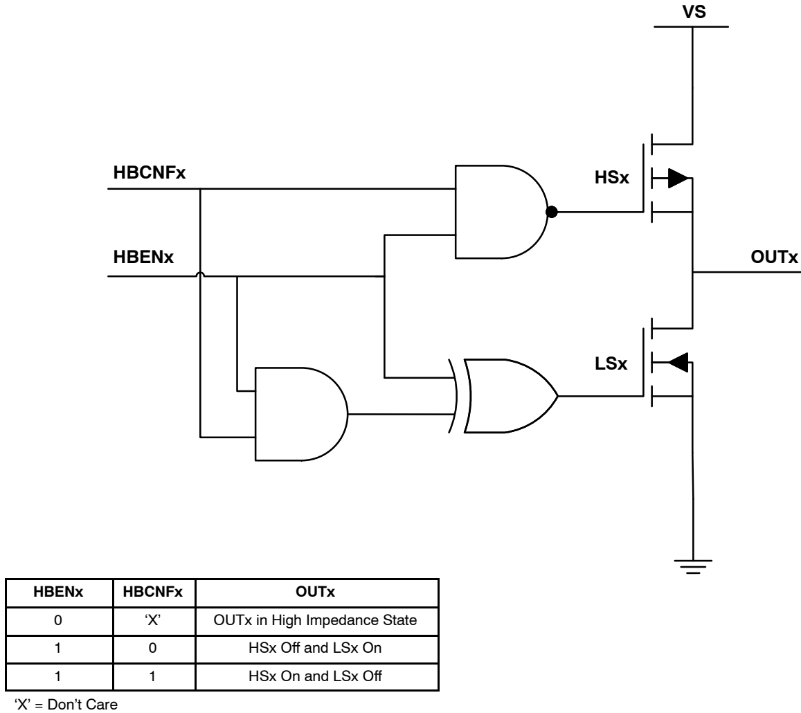
Figure 14. Bridge Control Logic
