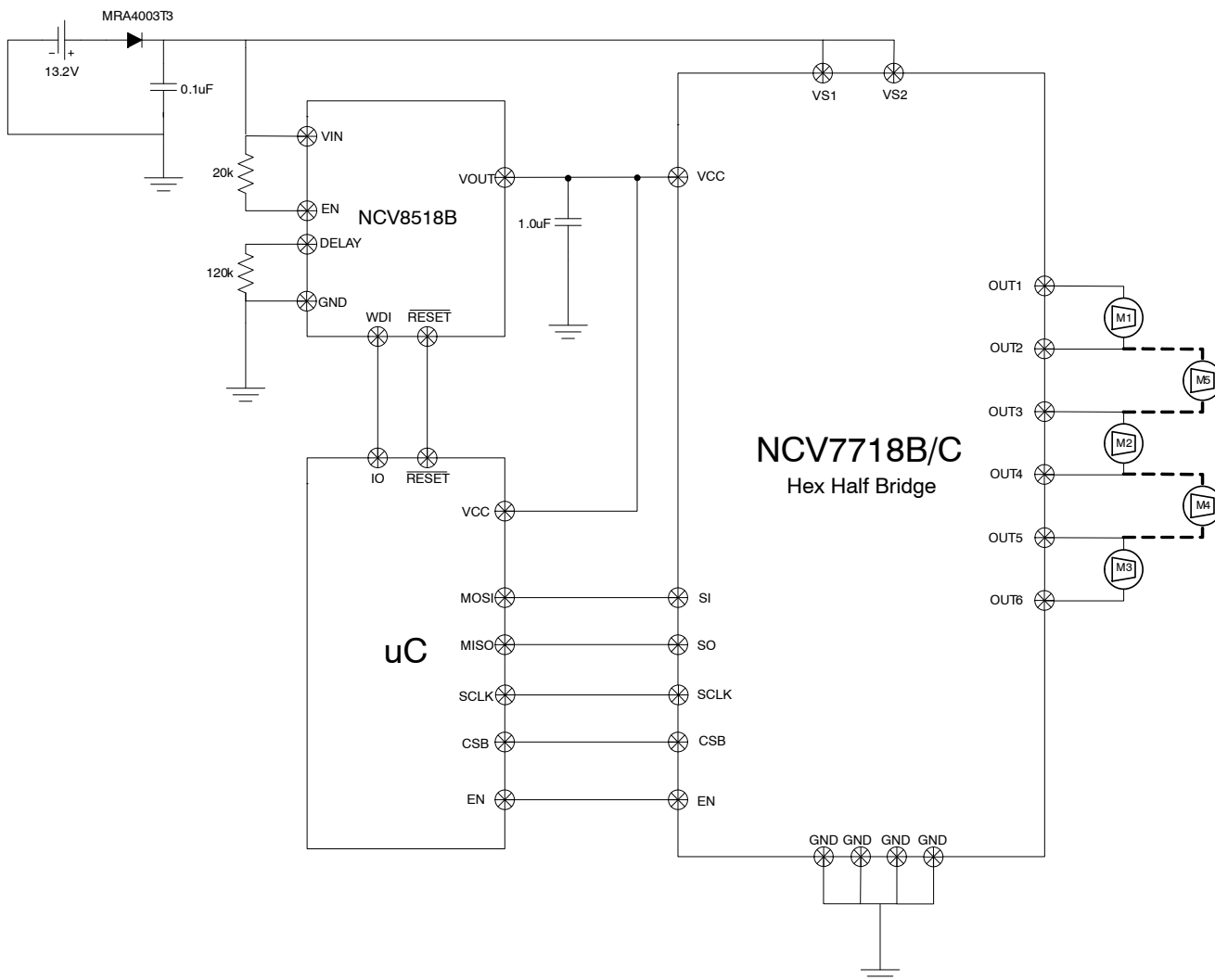
Figure 31. Application Drawing
