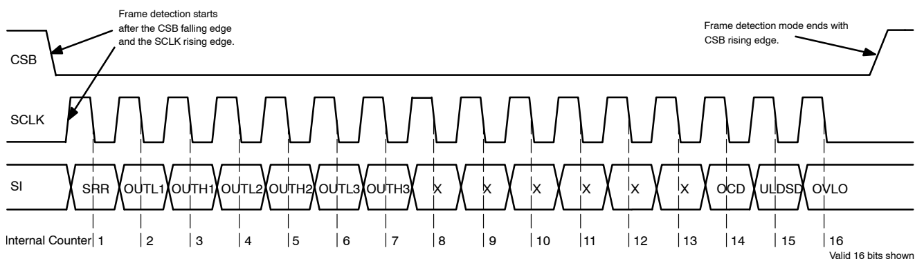
Figure 11. Frame Detection
