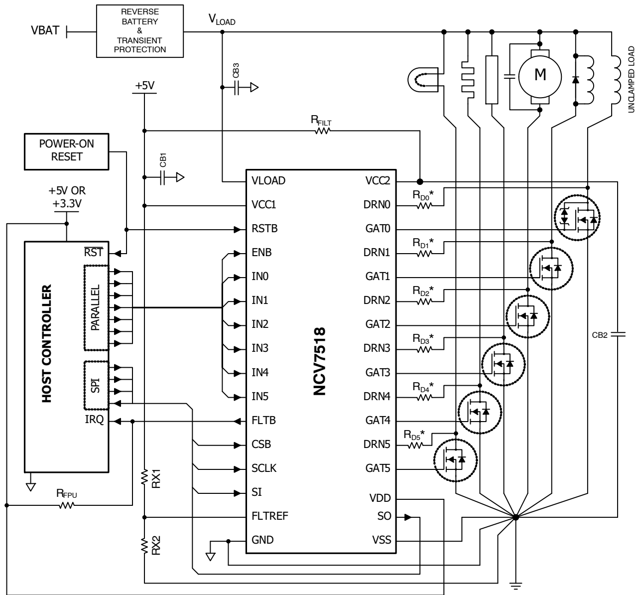
Figure 2. Application Diagram
