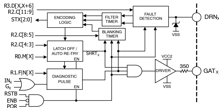
Figure 12. Gate Driver Channel
