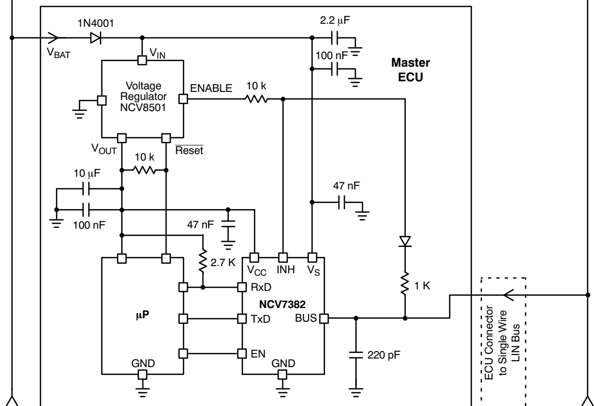
Figure 10. Application Circuitry
