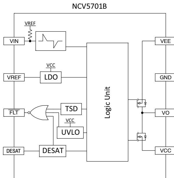
Figure 3(b). Simplified Block Diagram NCV5701B
