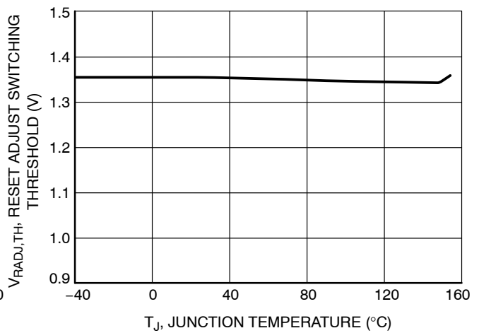
Figure 36. Reset Adjust Switching Threshold vs. Junction Temperature
