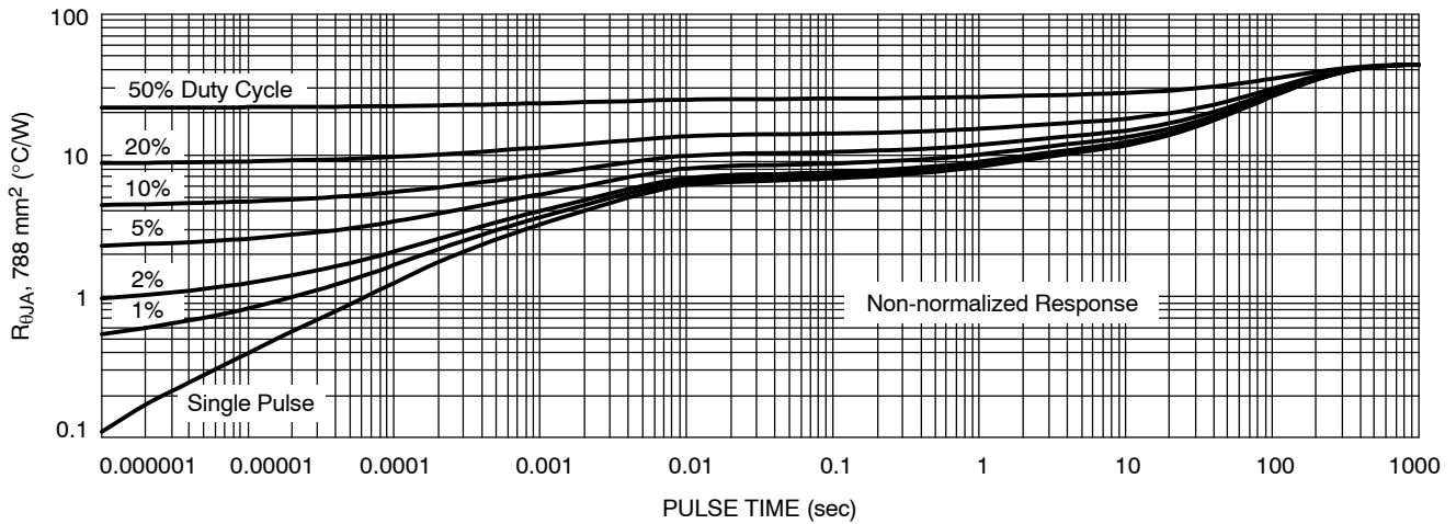
Figure 35. Duty Cycle for 1" Spreader Boards, D²PAK 5-Lead
