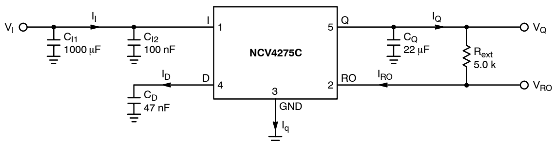
Figure 21. Test Circuit
