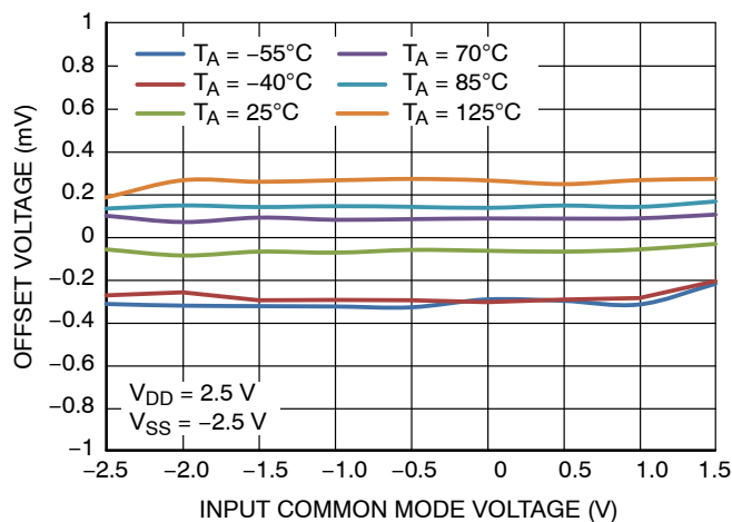
Figure 11. V_{OS} vs. V_{CM} ( V_S = 5\text{ V} )
