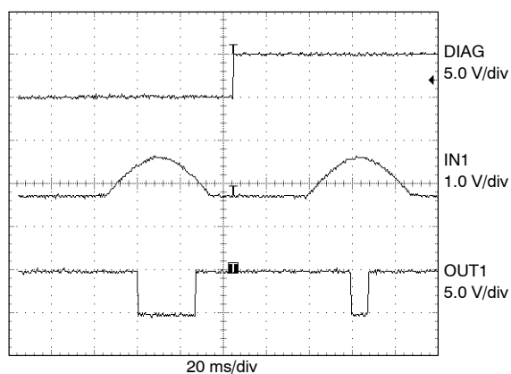
Figure 6. Diagnostic Operation
