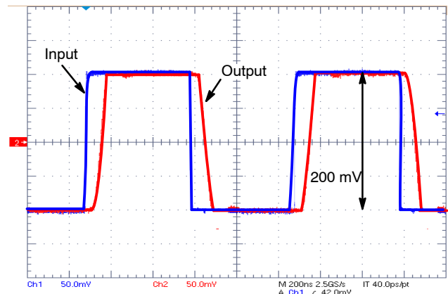
Figure 8. SD Small Signal Response
