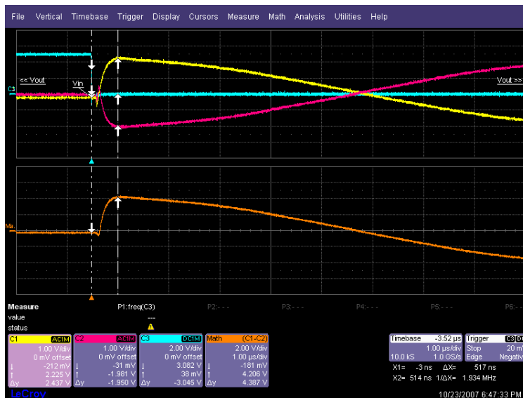
Figure 20. Turn-on Time
