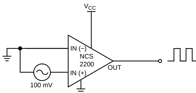
Figure 21. Zero-Crossing Detector
