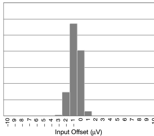
Figure 3d. Input Offset Voltage Distribution, G200
