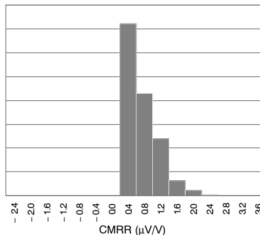
Figure 5a. Common Mode Rejection Ratio Distribution, G25
