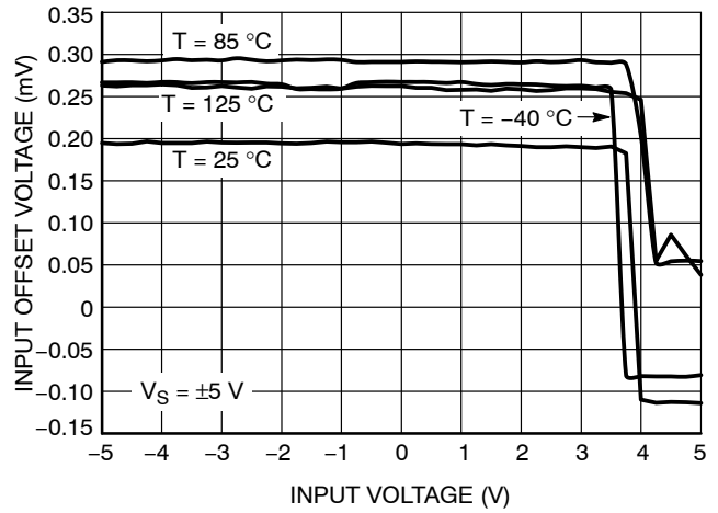
Figure 4. Input Offset Voltage vs. Common Mode Input Voltage
