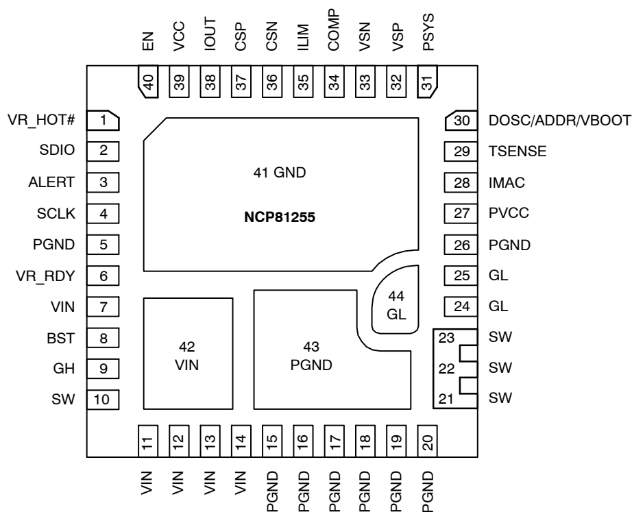
Figure 3. Pin Configuration
