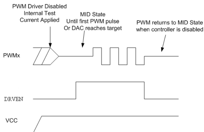
Figure 3. Soft-Start Sequence
