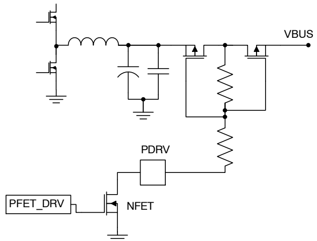
Figure 13. PFET Drive
