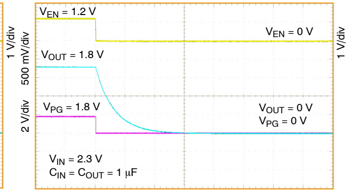
Figure 28. Turn-Off Response After De-asserting EN NCP752A/B, V_{OUT} = 1.8 V
