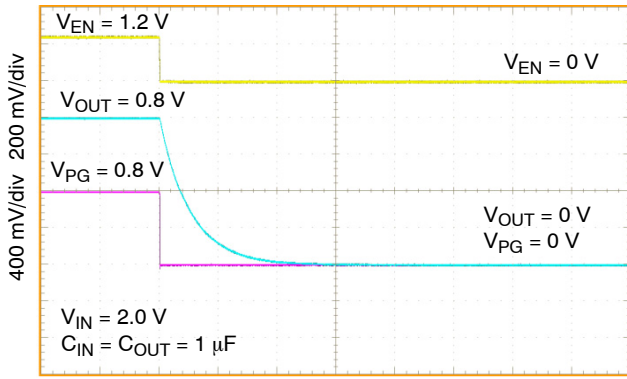
Figure 27. Turn-Off Response After De-asserting EN NCP752A/B, V_{OUT} = 0.8 V
