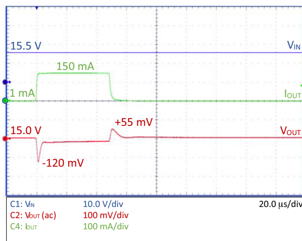
Figure 26. Load Transient – NCP730–15.0 V, C_{OUT} = 1\text{ }\mu\text{F}
