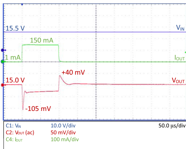
Figure 28. Load Transient – NCP730–15.0 V, C_{OUT} = 10\text{ }\mu\text{F}
