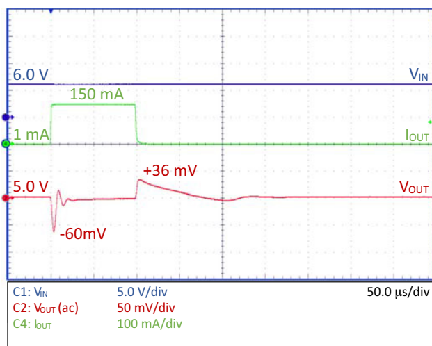
Figure 24. Load Transient – NCP730–5.0 V, C_{OUT} = 10\text{ }\mu\text{F}
