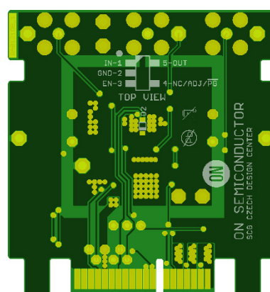
Figure 91. TSOP-5 Demo Board (2 layer, rev. 1) – PCB Bottom Layer
