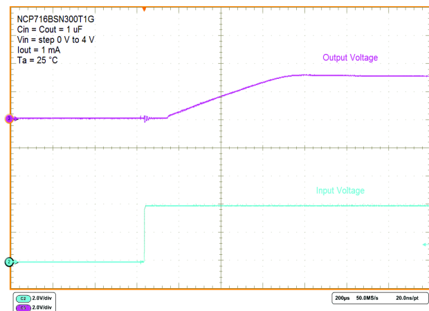
Figure 19. Turn-On Response
