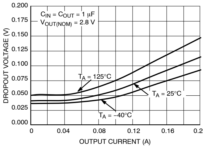
Figure 23. Dropout Voltage vs. Output Current V_{OUT} = 2.8 V
