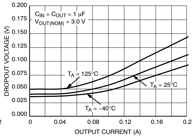
Figure 24. Dropout Voltage vs. Output Current V_{OUT} = 3.0 V
