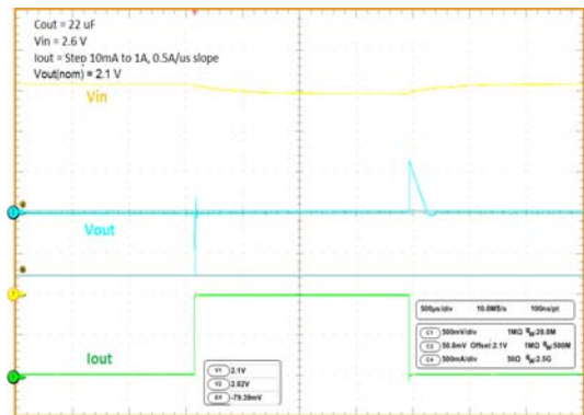
Figure 40. Load Transient Response
