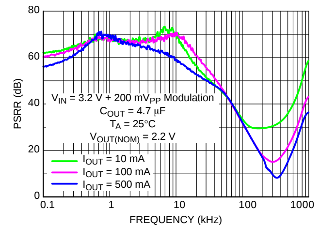
Figure 26. PSRR vs. Frequency & Output Current
