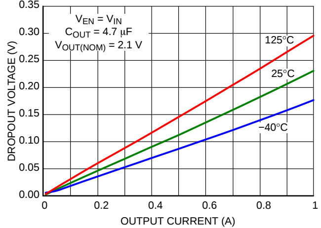
Figure 18. Dropout Voltage vs. Output Current
