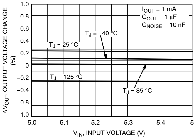
Figure 5. Line Regulation
