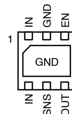
NCP691, NCP692 – DFN6
