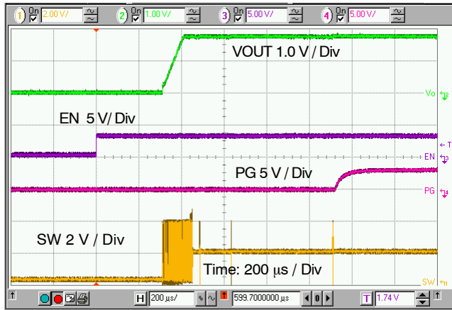
Figure 17. Power Up Sequence and Power Good ( V_{IN} = 3.6 V, V_{OUT} = 1.8 V, I_{OUT} = 0 A, L = 1 \mu H, C_{OUT} = 10 \mu F)
