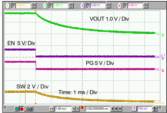
Figure 18. Power Down Sequence and Active Output Discharge ( V_{IN} = 3.6 V, V_{OUT} = 1.8 V, I_{OUT} = 0 A, L = 1 \mu H, C_{OUT} = 10 \mu F)
