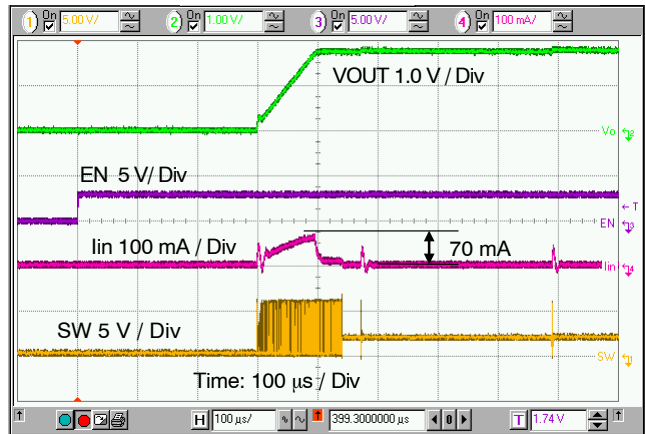
Figure 16. Power Up Sequence and Inrush Current in Input ( V_{IN} = 3.6 V, V_{OUT} = 1.8 V, I_{OUT} = 0 A, L = 1 \mu H, C_{OUT} = 10 \mu F)
