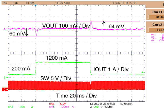
Figure 15. Load Transient Response ( V_{IN} = 3.6 V, V_{OUT} = 1.8 V, I_{OUT} = 200 mA to 1200 mA, L = 1 \mu H, C_{OUT} = 10 \mu F)
