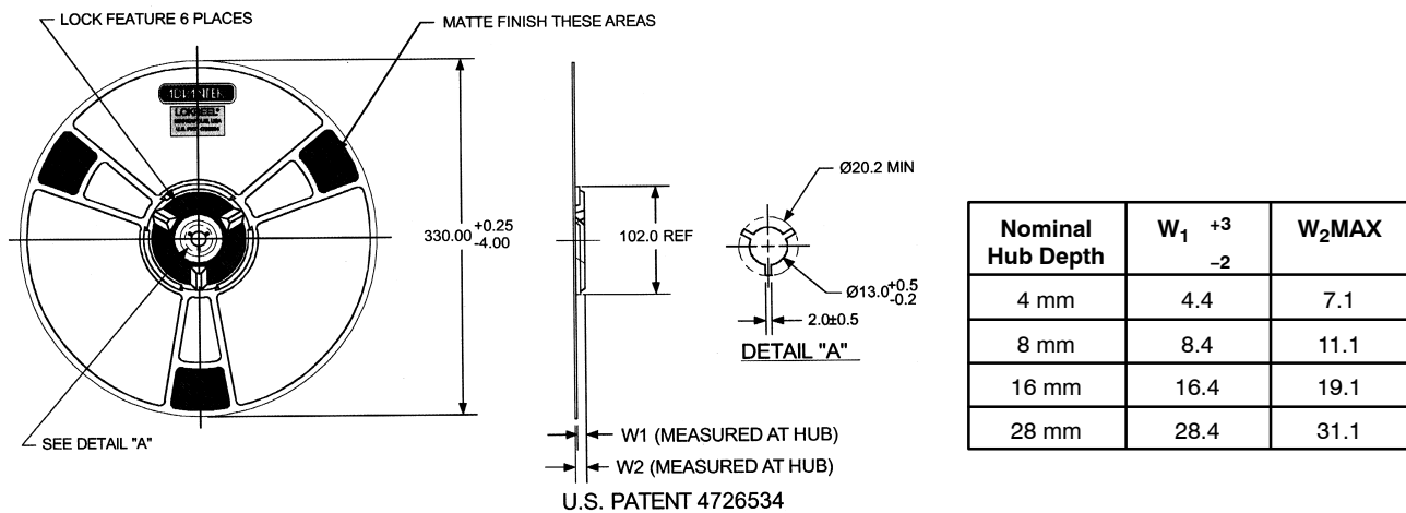
Figure 13. Reel Dimensions
