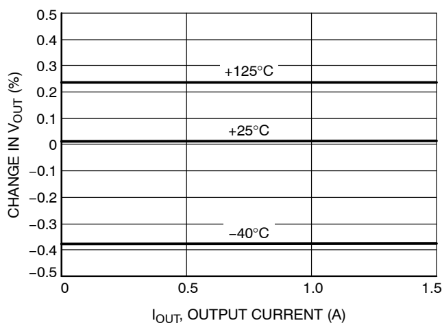
Figure 6. Load Regulation
