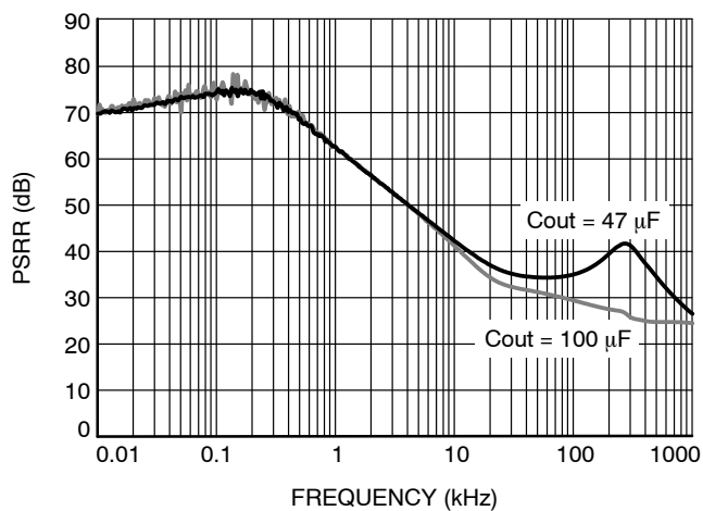
Figure 17. PSRR vs. Frequency, V_{in} = 3.5\text{ V} + 200\text{ mVpp} Modulation, V_{out} = 2.5\text{ V} , I_{out} = 0.5\text{ A}
