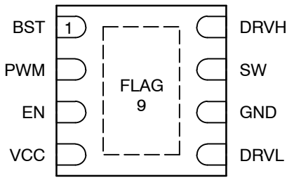
Figure 1. Pin Diagram
