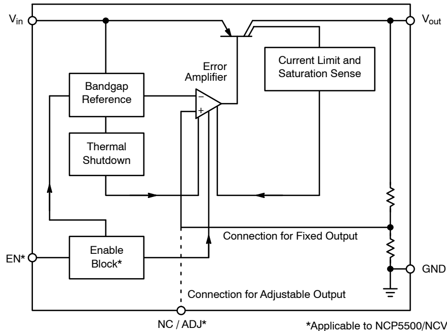
Figure 2. Block Diagram
