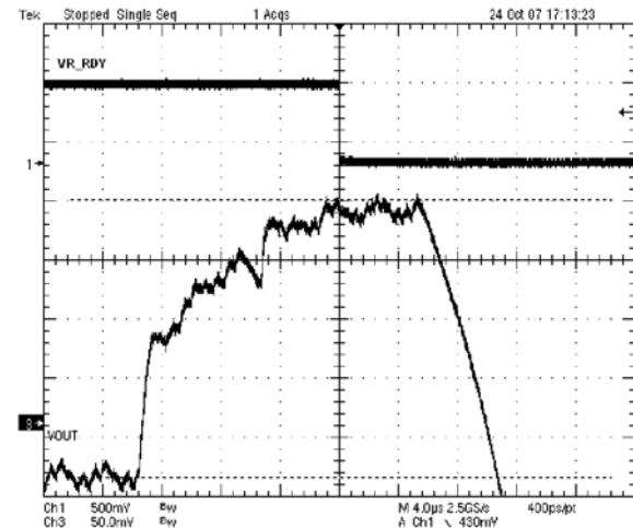
Figure 26. AMD, 1.55 V OVP Event
