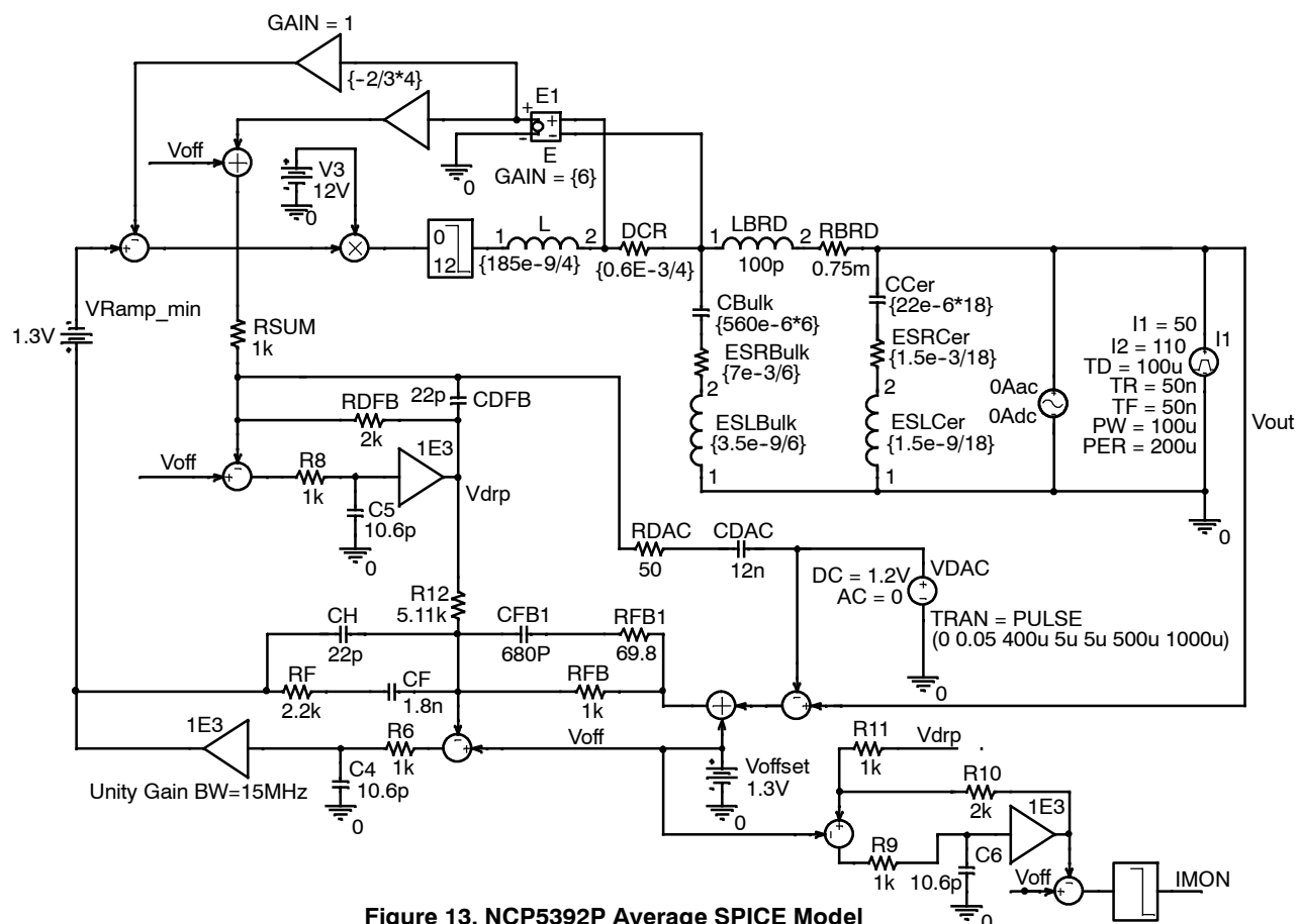
Figure 13. NCP5392P Average SPICE Model
