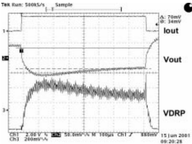
Figure 35. V_{\text{DRP}} Tuning, RC Time Too Long
