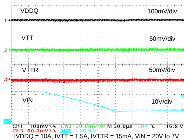
Figure 32. Line Transient 20V to 7V at Full Load
