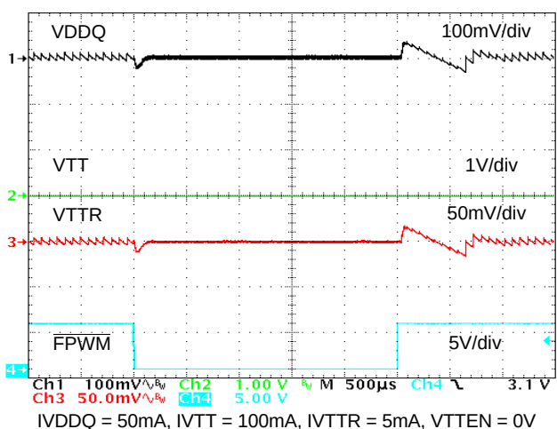
Figure 24. PS-FPWM-PS Transition Waveforms
