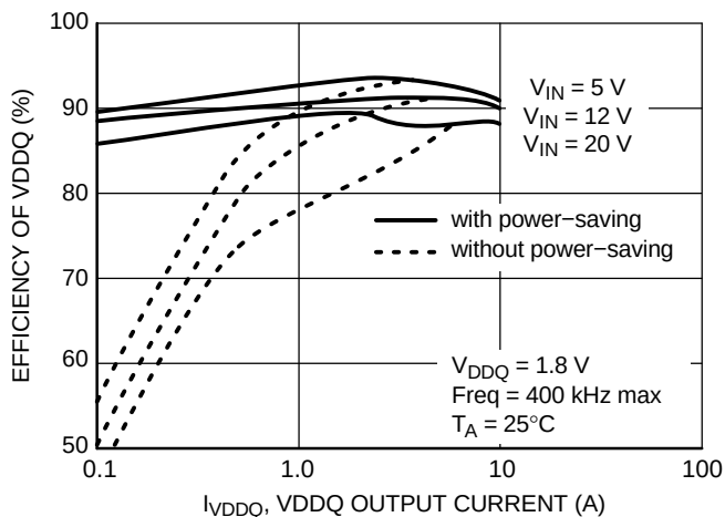
Figure 16. VDDQ Efficiency (DDR2) vs. VDDQ Output Current
