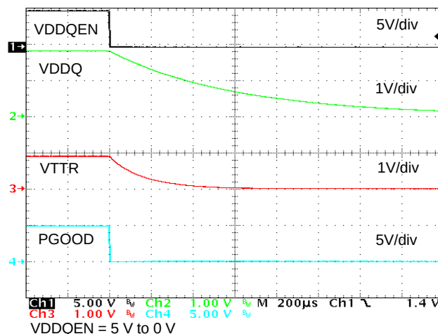
Figure 20. VDDQ, VTTR Shutdown Waveforms
