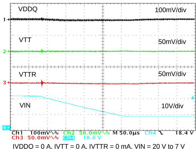
Figure 30. Line Transient 20V to 7V at No Load
