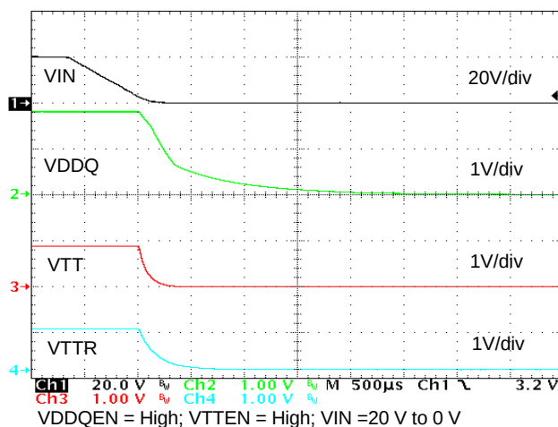
Figure 18. Power-Down Waveforms
