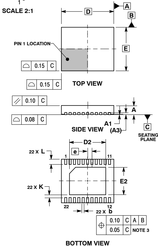
DFN22 6x5x0.9 MM, 0.5 P CASE 506AF ISSUE A
