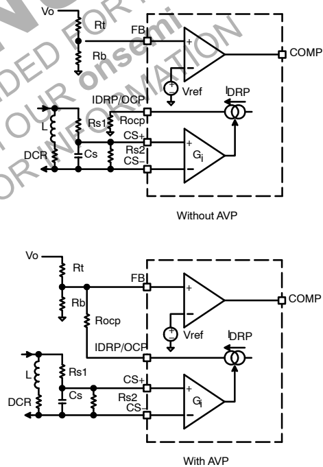
Figure 24. OCP Configuration
