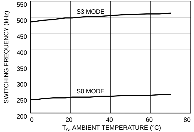
Figure 4. Oscillation Frequency in S0/S3 vs. Ambient Temperature
