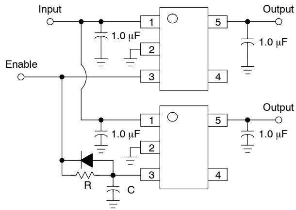
Figure 32. Delayed Turn-on
