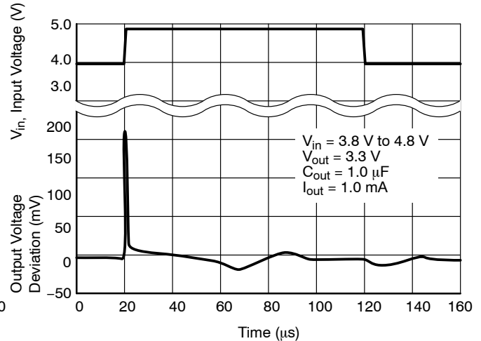
Figure 19. Line Transient Response
