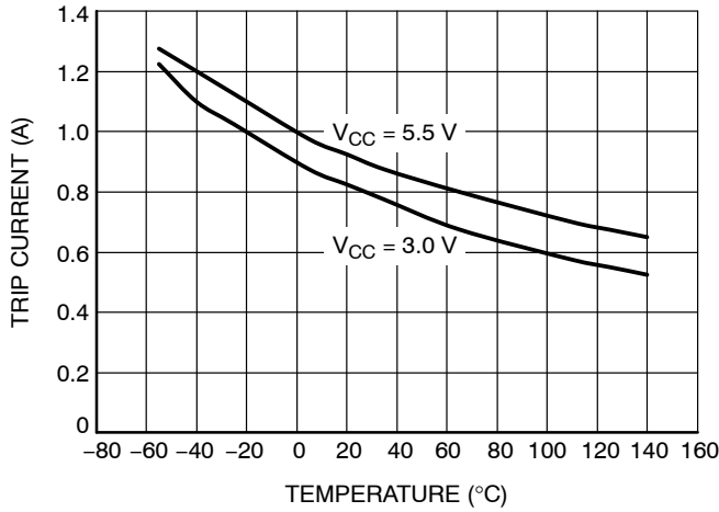
Figure 21. OCP Trip Current vs. Temperature
