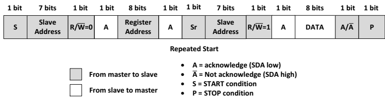
Figure 7. I 2 C Read with Repeated Start Format
