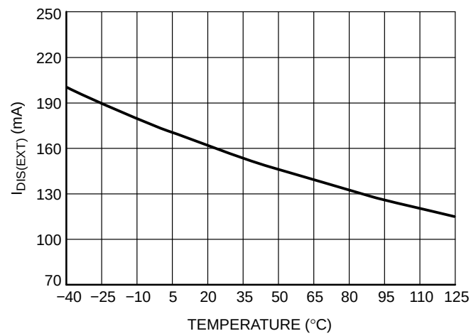
Figure 15. VCC Discharge Current, I_{DIS(EXT)}
