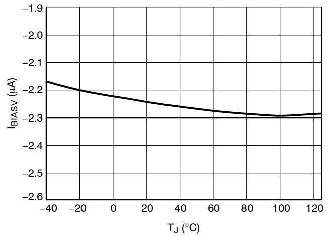
Figure 13. IBIASV at V CC = 15 V, V SNS > V SNSBIASHT
