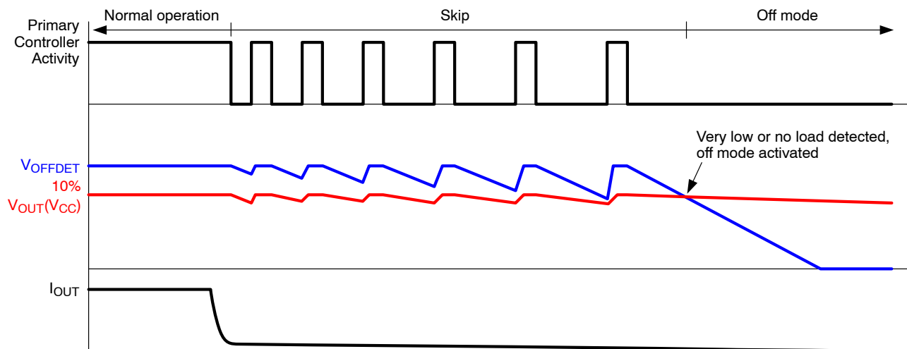
Figure 27. OFF Mode Detection
