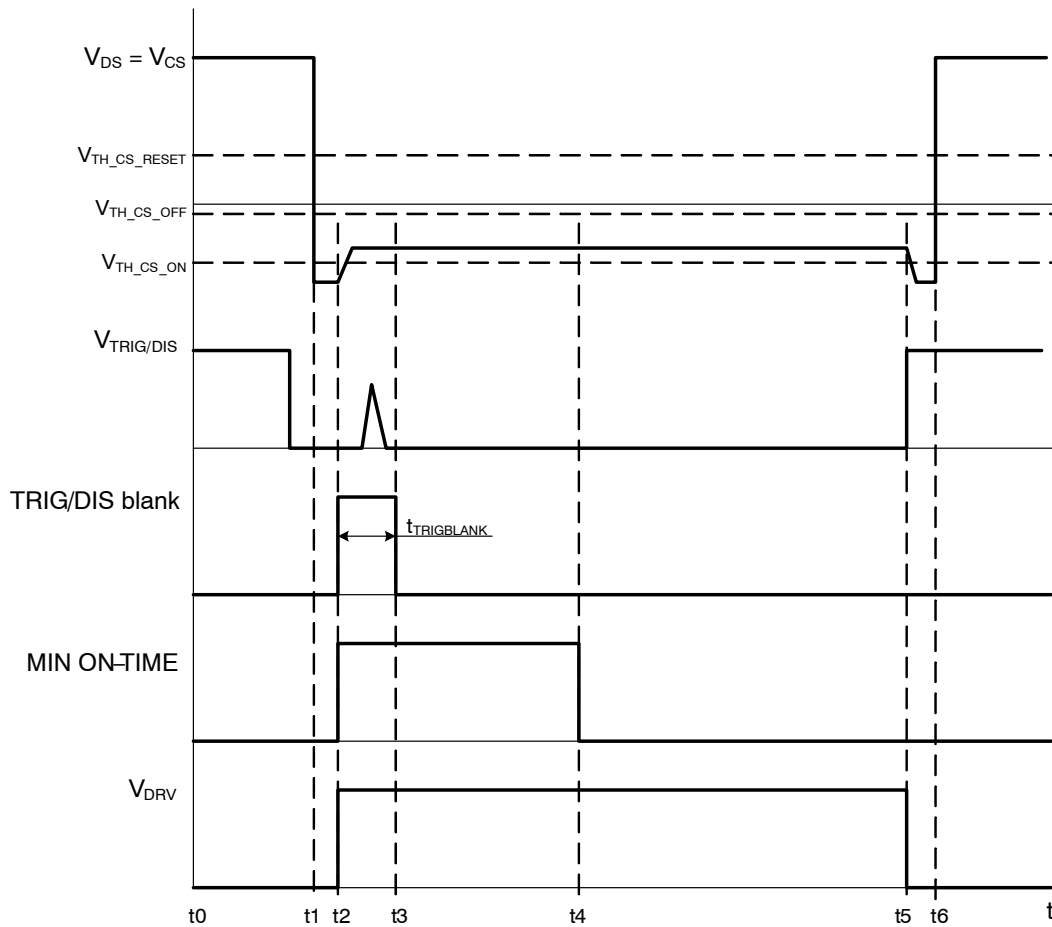
Figure 54. Trigger Input Functionality Waveforms – Trigger Blanking Acts Like a Filter
