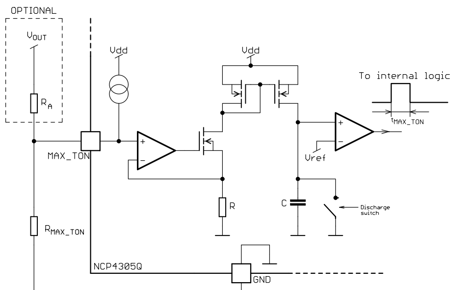
Figure 72. Internal Connection of the MAX TON Generator, NCP4305Q
