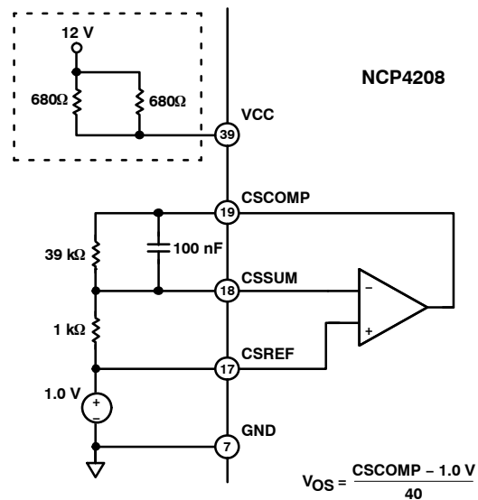
Figure 6. Positioning Voltage
