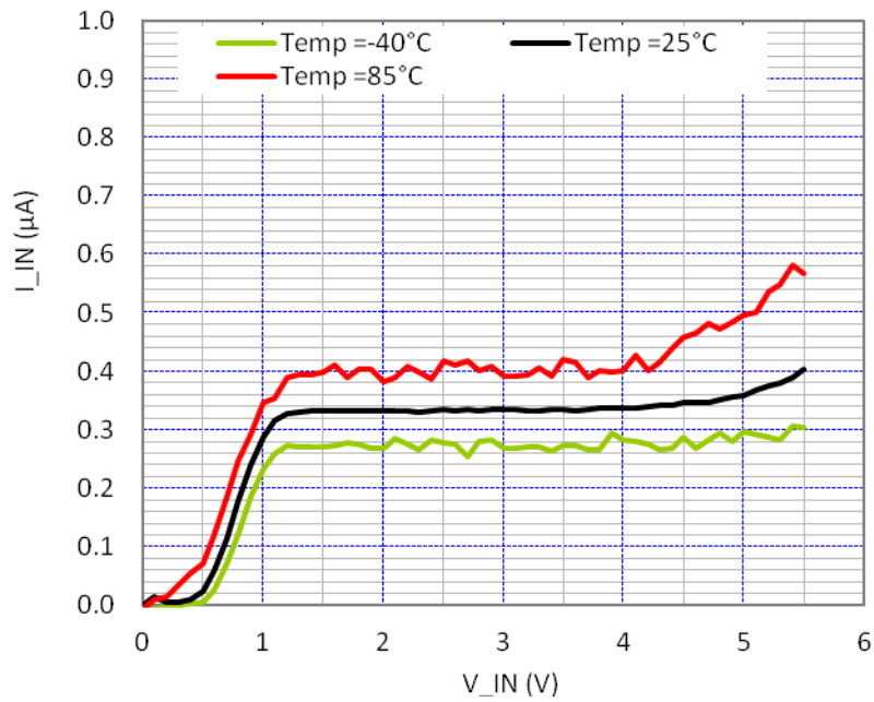
Figure 4. Standby Current (μA) versus Vin (V)
