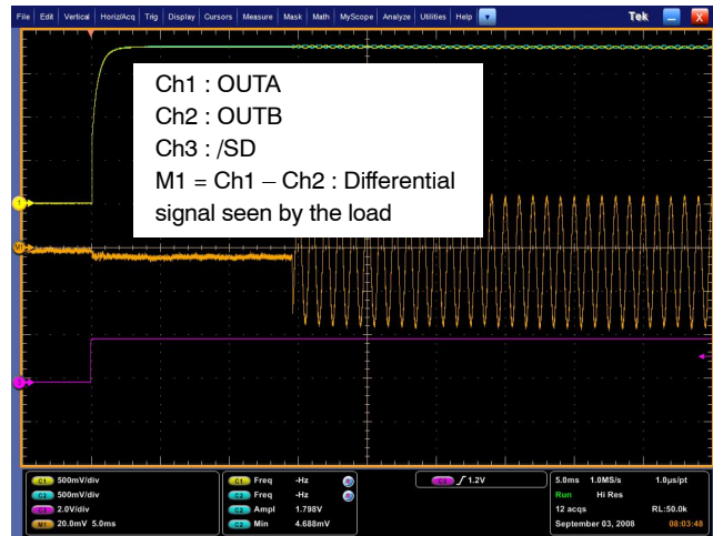
Figure 34. Zero pop noise turn on sequence with single-ended input audio source ( C_i = 47 \text{ nF} , R_i = 24 \text{ k}\Omega , R_f = 24 \text{ k}\Omega , C_{byp} = 1 \mu\text{F} , R_l = 8 \Omega , T_{on} = V_p )
