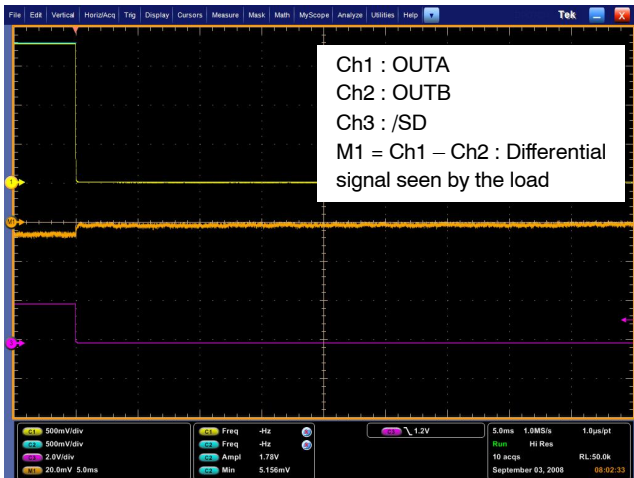
Figure 35. Zero pop noise turn off sequence with single-ended input to ground ( C_i = 47 \text{ nF} , R_i = 24 \text{ k}\Omega , R_f = 24 \text{ k}\Omega , C_{byp} = 1 \mu\text{F} , R_l = 8 \Omega , T_{on} = V_p )
