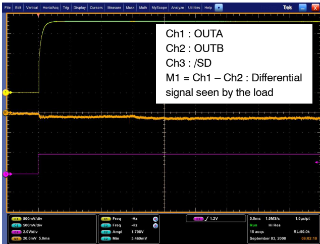
Figure 33. Zero pop noise turn on sequence with single-ended input to ground ( C_i = 47 \text{ nF} , R_i = 24 \text{ k}\Omega , R_f = 24 \text{ k}\Omega , C_{byp} = 1 \mu\text{F} , R_l = 8 \Omega , T_{on} = V_p )
