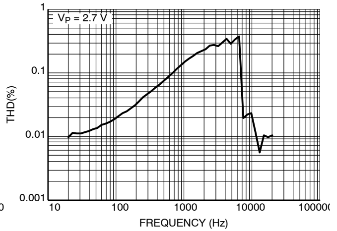
Figure 10. THD+N vs Frequency P_{out} = 300\text{ mW} , R_L = 4\ \Omega
