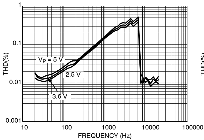
Figure 7. THD+N vs Frequency P_{out} = 250 \text{ mW} , R_L = 8 \Omega
