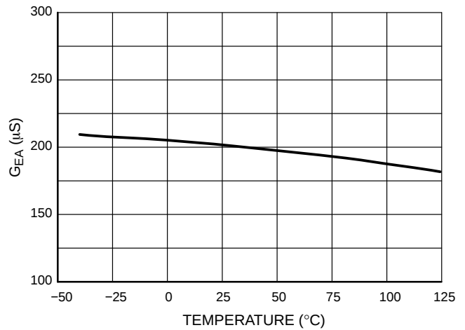
Figure 17. G_{EA} vs. Temperature
