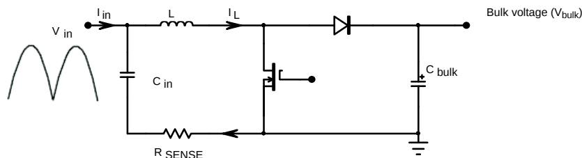
Figure 41. CCM PFC Boost Converter
