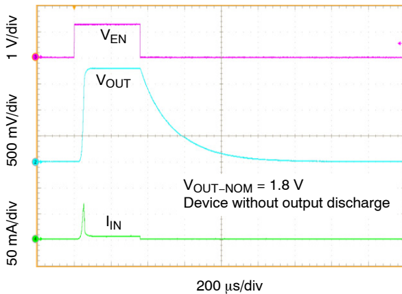
Figure 29. Turn-ON/OFF – V_{EN} driven
