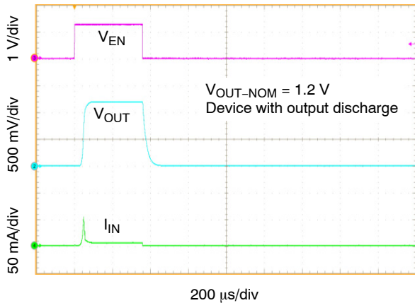
Figure 28. Turn-ON/OFF – V_{EN} driven
